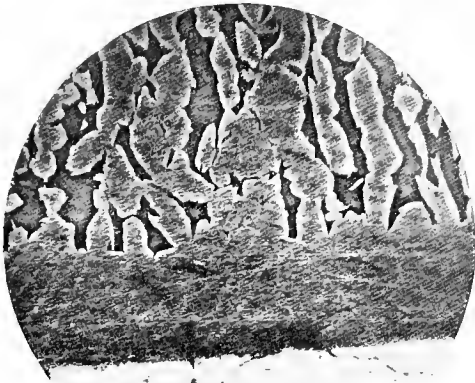
A. Diffusion of zinc into copper. \times 30 .
